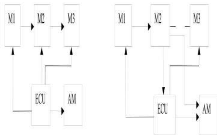
Figure 1. layout of FMS and layout with third machine (M3) breakdown
