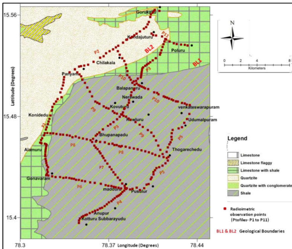
Figure 1 Layout map of the Radiometric survey, overlaid on the geological map of the study area (modified after GSI, 2005).
