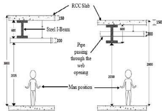
Figure 4-1 - Reduction in height of building storeys, Morkhadeet. al. 2019[4].
