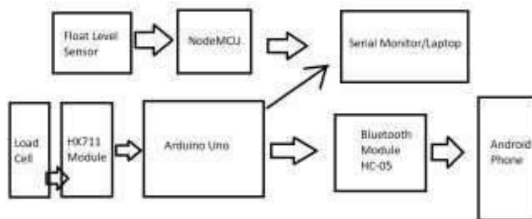
Fig. 1 Block schematic
