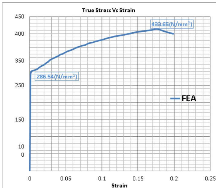
Figure 8 FEA result true stress vs strain
