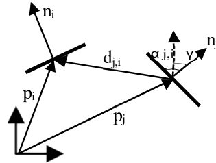
Figure 2 Local convexity
