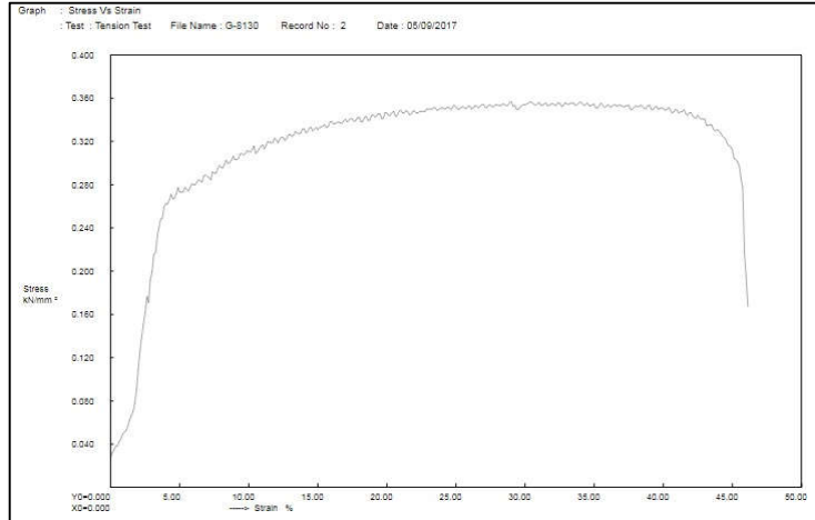
Figure 5 Experimental result stress vs strain
